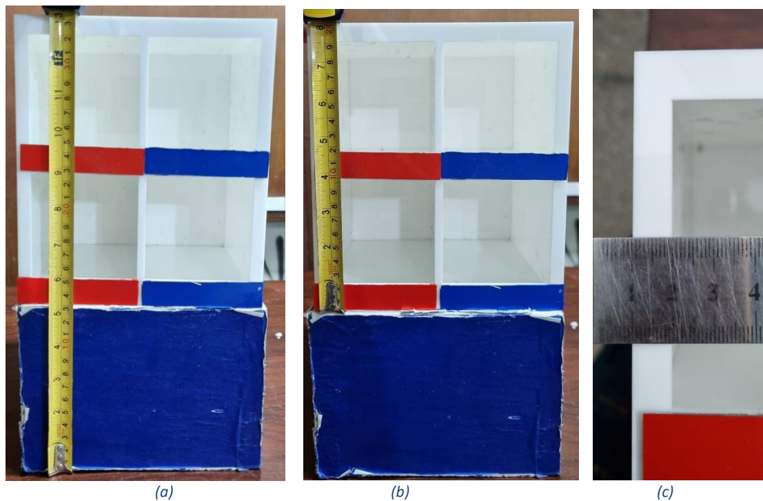
Figure 1: Storage Box. (a) Height of storage box assembly 13 inches, (b) Height of storage box 7 inches, (c) Distance from the outer boundary of the storage box to the slot opening
