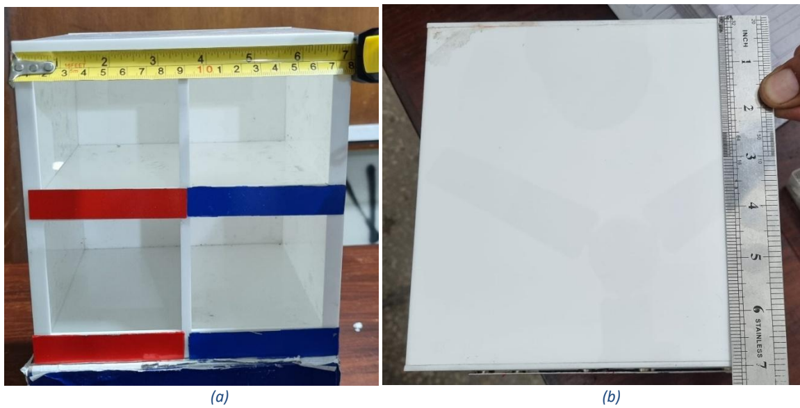
Figure 3: Storage Box. (a) Width of storage box 7 inches, (b) Depth of storage box 7 inches
