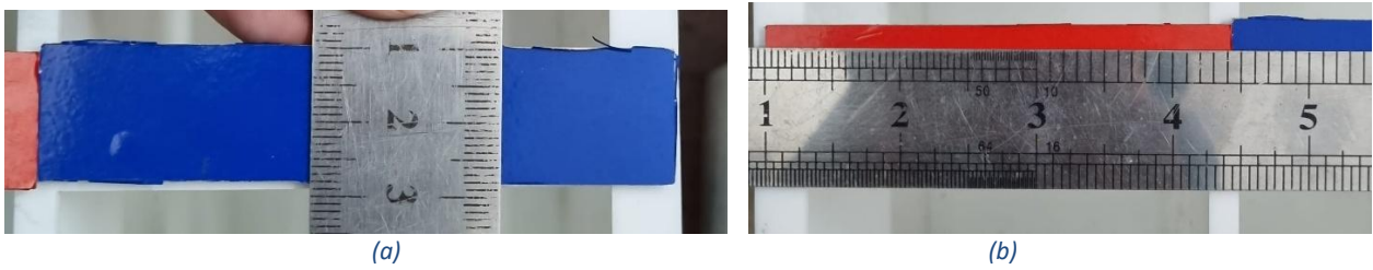
Figure3: Colored Strip. (a) Width of colored strip 0.75", (b) Length of colored strip 3.5"
